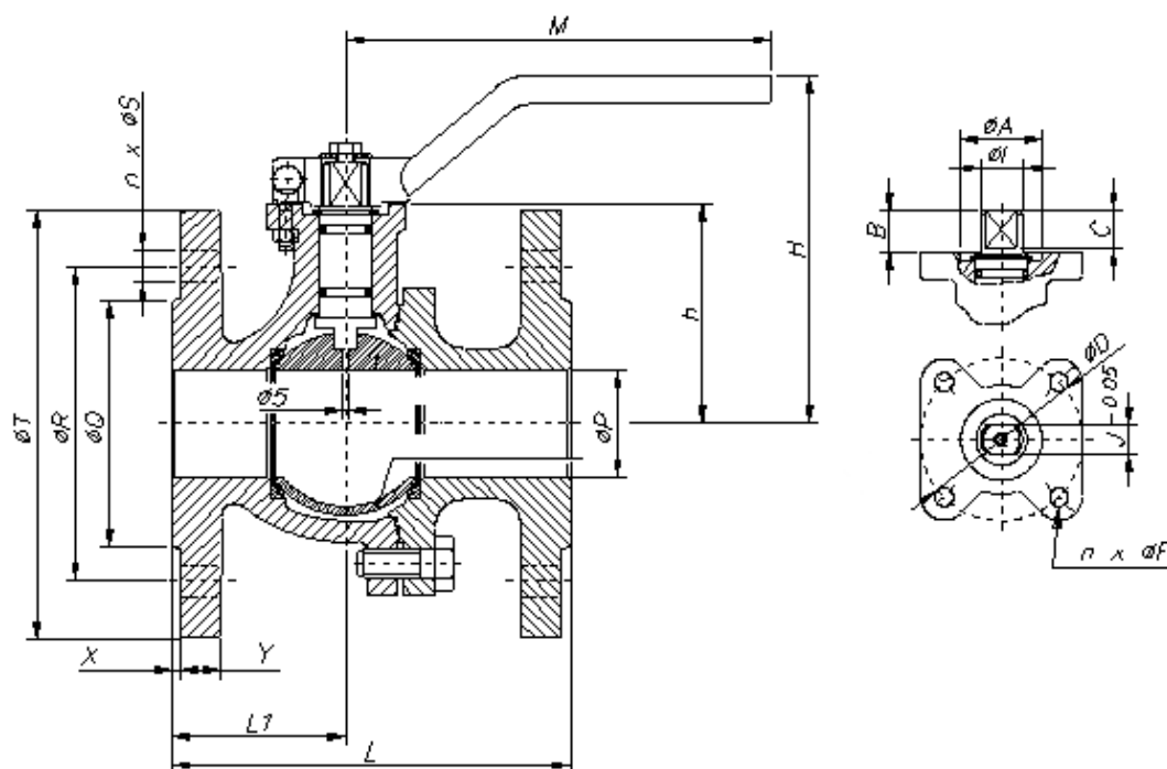
DIMENSIONS: (mm)
